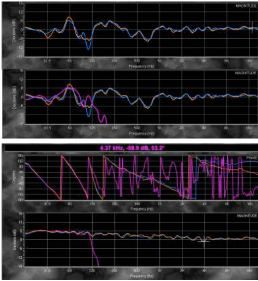
Top: Typical frequency response of stand-mounted near-field monitors behind console before and after PFS implementation
